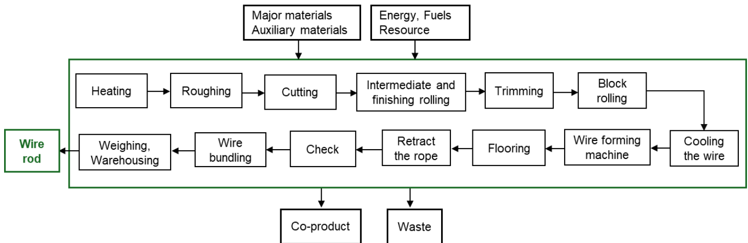
Wire rod production of Hung Yen Plant
